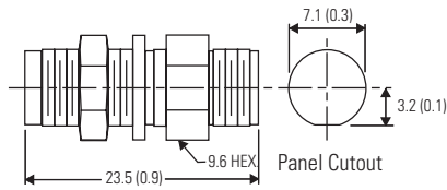
Bulkhead Adapter Dimensions (2090-S-BLHD)
