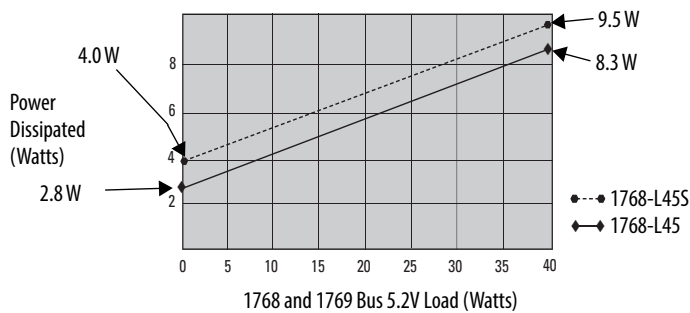
Figure 11 - 1768-L45 and 1768-L45S Power Dissipation
